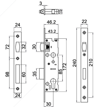
MTS RL DL84030 GUN METAL
