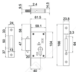
MTS SLD DL 84100N BLACK PEARL
