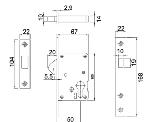
MTS SLD DL 85100 GUN METAL
