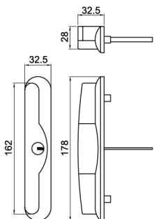
J8C WITH LOCK WH Available : BK
